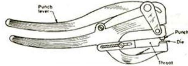
Fig. 15-8, Hand lever punch.
